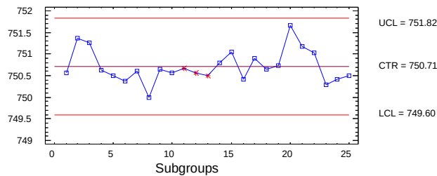
Figure (1): X –bar chart based on (\hat{\sigma})
