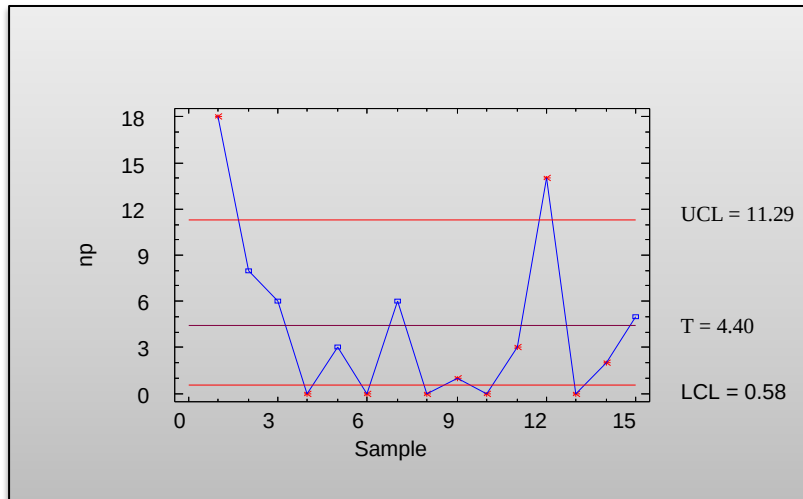
Figure 3: Number of Defectives chart based on regression equations
